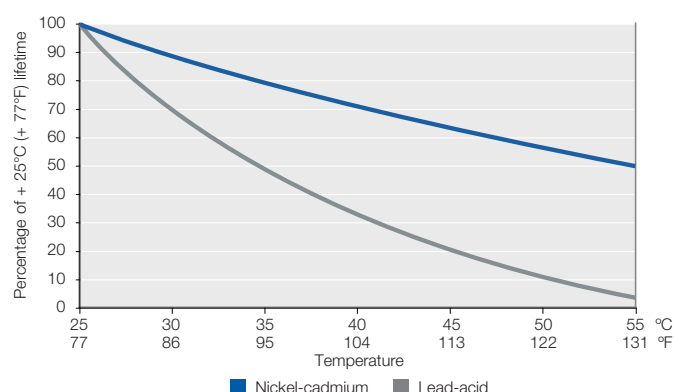
Effect of temperature on lifetime
